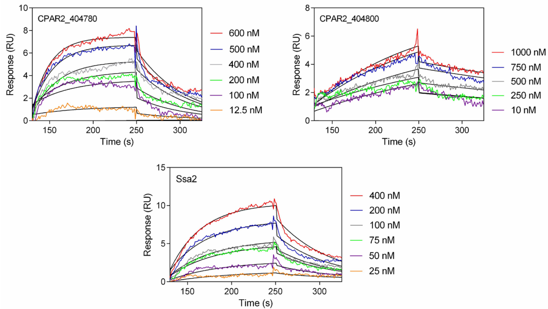
Figure 5. SPR sensograms representing interactions between HPG and CPAR2_404780, CPAR2_404800 and Ssa2. SPR characteristics of the interaction between the HPG and a particular fungal protein immobilized onto a surface of the CM5 chip. The global data fits with the Langmuir 1:1 binding model (with a baseline drift) are shown as black lines. The HPG solutions at a concentration range of 10–1000 nM were injected at a flow rate of 30 \mu l/min for 120 seconds.
