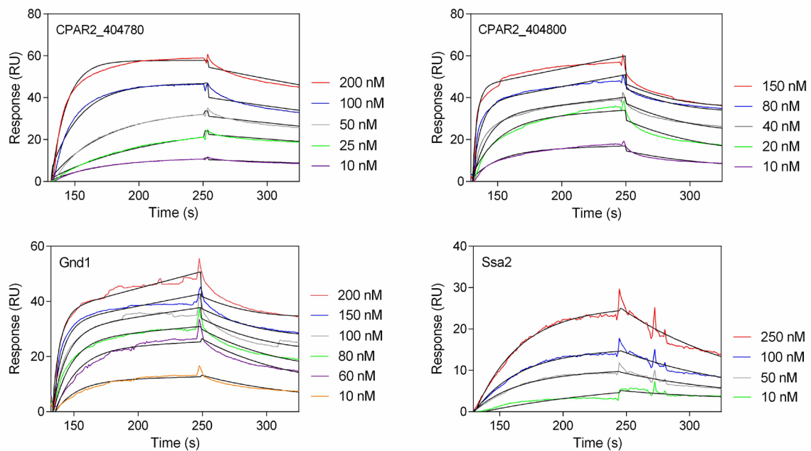
Figure 6. HK binding by CPAR2_404780, CPAR2_404800, Ssa2 and Gnd1 investigated by SPR measurements. Interactions between HK and individual fungal protein presented as the entire sets of SPR sensograms obtained during the injection of HK solutions at a concentration range of 10–250 nM at a flow rate of 30 \mu l/min for 120 seconds over the surface of the CM5 chip with immobilized C. parapsilosis individual protein. Black lines illustrate the global data fits with the Langmuir 1:1 binding model (with a baseline drift).
