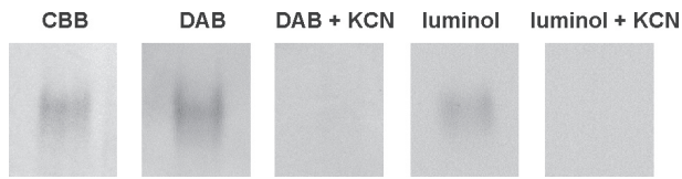
Figure 1. Analysis of peroxidase activity of rMhb1
