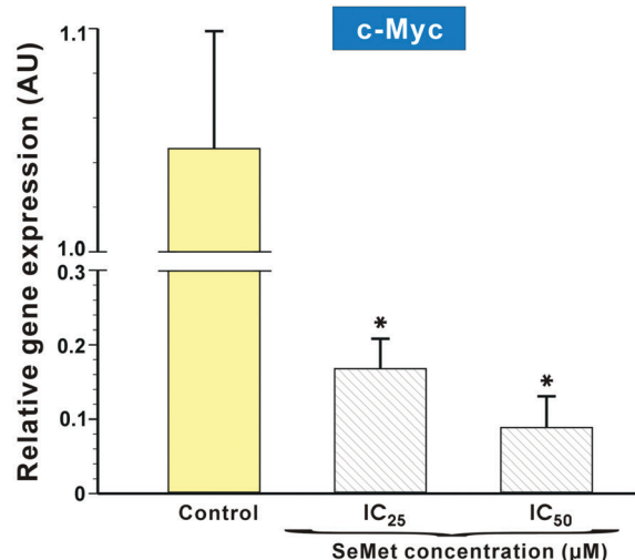
Figure 6. Effect of SeMet stimulation on c-Myc gene expression. HT-29 cells were incubated with cytotoxic doses (IC 25 , IC 50 ) of SeMet for 48 h and mRNA was analysed by qPCR. SeMet significantly decreased c-Myc gene expression in HT-29 cells with respect to the untreated control. Experiments were performed in quadruplicates and quantified using HPRT as a reference gene. Data are shown as the mean \pm S.D. and are representative of three independent experiments. * P < 0.05 determined by Student's t -test.
