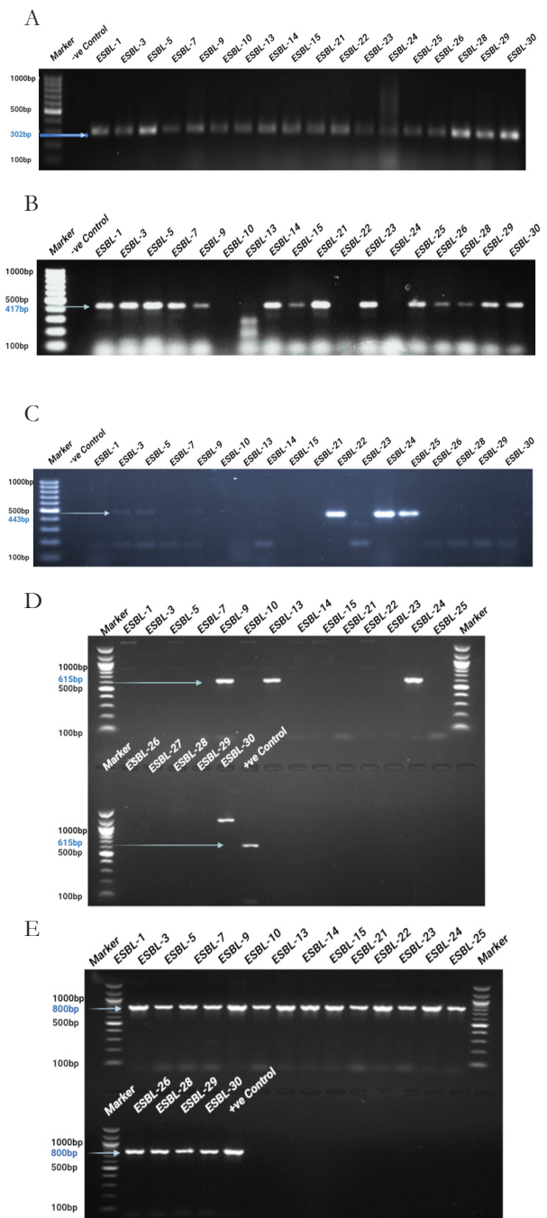
Figure 3. PCR amplification of ESBL traits. Figure 3A: bla_{CTX-M15r} Figure 3B: bla_{CMY-2r} Figure 3C: bla_{NDM-1r} Figure 3D: bla_{NDM-1r} Figure 3 E: bla_{TEM-1r} . Amplicons, prepared as described in Methods and in Table 1, were loaded on the gel in the following order: in Fig. 3A, 3B and 3C; Lane 1 M -100 bp ladder. Lane 2: Negative control, Lane 3 ESBL 1, Lane 4 ESBL3, Lane 5 ESBL 5, Lane 6 ESBL 7, Lane 7 ESBL 9, Lane 8 ESBL 10, Lane 9 ESBL13, Lane 10 ESBL 14, Lane 11 ESBL 15, Lane 12 ESBL 21, Lane 13 ESBL 22, Lane 14 ESBL 23, Lane 15 ESBL 24, Lane 16 ESBL 25, Lane 17 ESBL 26, Lane 18 ESBL 28, Lane 19 ESBL 29, Lane 20 ESBL 30. Loading order for Fig. 3D and 3E; Top Panel: Lane 1 100 bp ladder, Lane 2 ESBL 1, Lane 3 ESBL 3, Lane 4 ESBL 5, Lane 5 ESBL 5, Lane 6 ESBL 7, Lane 7 ESBL 10, Lane 8 ESBL 13, Lane 9 ESBL 14, lane 10 ESBL 15, Lane 11 ESBL 21, Lane 12 ESBL 23, Lane 13 ESBL 23, Lane 14 ESBL 24, Lane 15 ESBL 25, Lane 16 100 bp ladder. Bottom Panel: Lane 1 100 bp DNA ladder, Lane 2 ESBL 26, Lane 3 ESBL 28, Lane 4 ESBL 29, Lane 5 ESBL 30 and Lane 6 Positive control.
