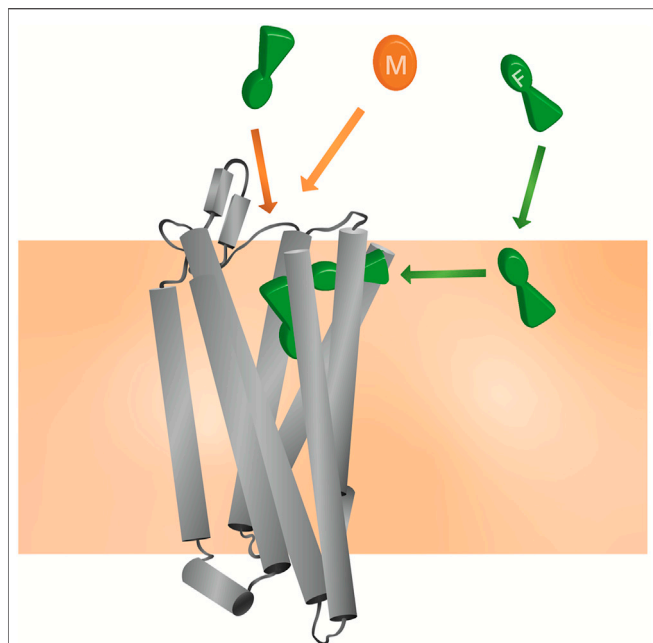
FIGURE 8 | Model for the unique pharmacology of fentanyl at the MOPr. In competition with a morphinan ligand (such as morphine or naloxone), fentanyl (green) can access the orthosteric pocket via two binding routes; the canonical aqueous pathway and by the novel lipid pathway. In contrast, the morphinan ligand (orange) only has access to one binding route.
