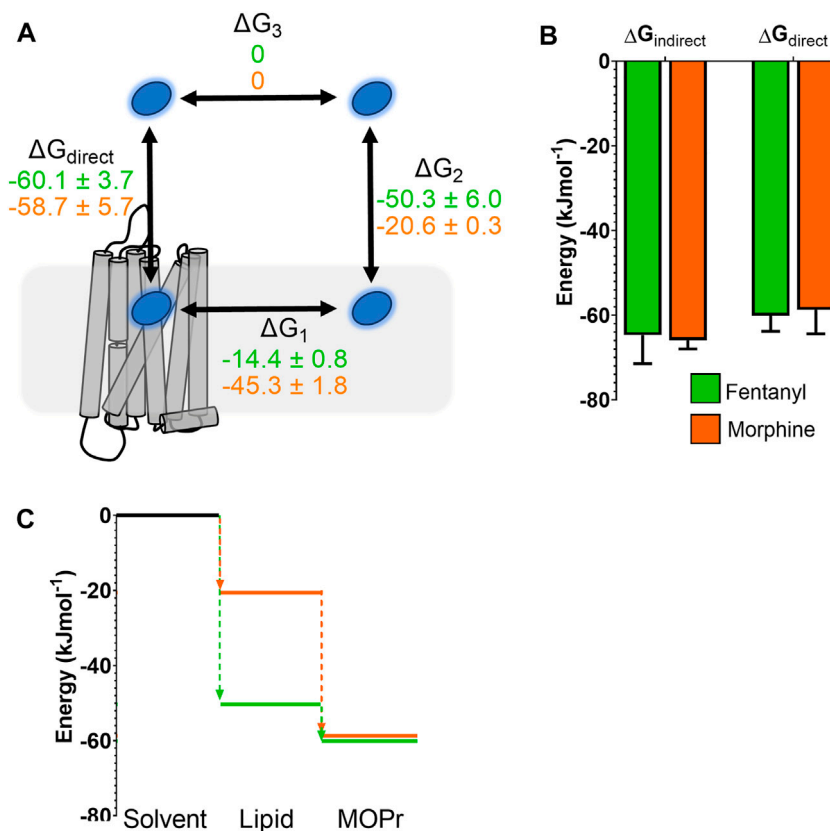
FIGURE 6 | Comparison of free energy landscapes for fentanyl and morphine binding to the MOPr. (A) Thermodynamic cycle for opioid ligand binding to MOPr; either by the direct, aqueous pathway ( \Delta G_{\text{direct}} ) or via the lipid membrane ( \Delta G_1 + \Delta G_2 ). Values for protonated fentanyl (green) and protonated morphine (orange) are taken from the PMF calculations in Figures 1D, 5 . Diffusion through the solvent ( \Delta G_3 ) is assumed to be 0. (B) Comparison of the free energy of binding to MOPr directly via the aqueous solvent, or indirectly via the membrane, where \Delta G_{\text{indirect}} = \Delta G_1 + \Delta G_2 + \Delta G_3 . (C) 2D representation of the indirect, lipid binding route, using the same values as (A) . Fentanyl (green) has a greater propensity to move into the lipid from the solvent, than morphine (orange).
