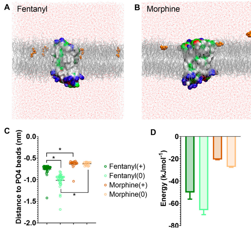
FIGURE 1 | Differences in how opioid ligands partition into the lipid bilayer. (A) Fentanyl molecules (orange) rapidly partitioned into the lipid membrane (grey). (B) Morphine molecules (orange) did not fully enter the lipid membrane (grey) but interacted with the charged lipid headgroups. Note while ligands can appear on either side of the bilayer due to the periodic boundary conditions applied in these simulations, for clarity only ligands in the upper leaflet of the membrane are shown. In no simulation did a ligand travel all the way through the bilayer. The protein is coloured according to residue properties (hydrophobic; grey, polar; green, acidic; red, basic; blue). (C) Distance between the center of mass of the ligand and the phosphate head groups (PO4 beads) of the lipid bilayer. Both the charged and neutral forms of fentanyl partitioned significantly deeper in the membrane than morphine. * p < 0.05 , one-way ANOVA. Each data point represents the average distance between a fentanyl molecule and the PO4 beads over the entire simulation. (D) Free energy change for ligands moving between the bilayer center and the aqueous solvent. Calculated from PMF profiles shown in Supplementary Figure S3 . Data plotted as mean \pm error calculated from bootstrap analysis.
