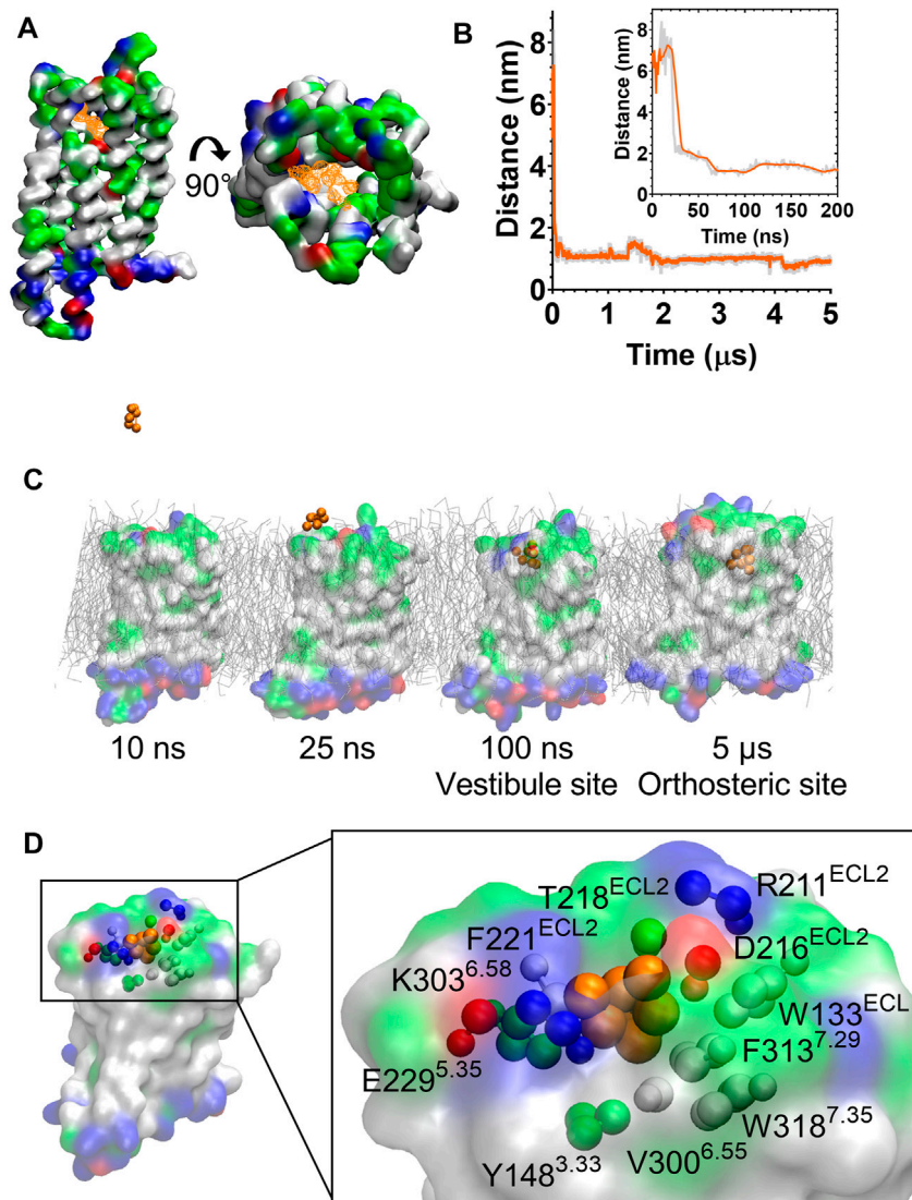
FIGURE 4 | Morphine binds to the MOPr from the aqueous phase, via an extracellular vestibule site. (A) Ligand density maps averaged over the 5 \mu s simulation, show morphine densities above and within the orthosteric pocket (orange). The protein is coloured according to residue properties (hydrophobic; grey, polar; green, acidic; red, basic; blue). (B) Distance between the Qd bead of morphine and the SC1 bead of D147 3,32 over the entire 5 \mu s and in the first 200 ns (inset). Data are presented as the raw values (grey) and moving average over 10 frames (orange). (C) Snapshots from the unbiased simulation of morphine binding to MOPr. Morphine moved from the aqueous solvent to an extracellular vestibule and finally the orthosteric site. (D) Morphine in the extracellular vestibule site. Morphine is depicted as orange beads, and the residues comprising the vestibule site as coloured beads.
