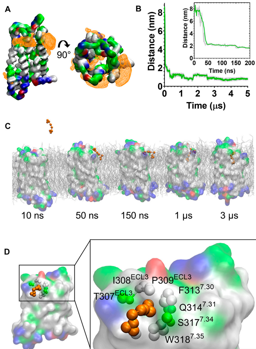
FIGURE 3 | Fentanyl binds to the MOPr from the lipid phase, via a gap between TM6 and TM7. (A) Ligand density maps averaged over the 5 \mu s simulation, show fentanyl densities around the receptor transmembrane domains and within the orthosteric pocket (orange). The protein is coloured according to residue properties (hydrophobic; grey, polar; green, acidic; red, basic; blue). (B) Distance between the Qd bead of fentanyl and the SC1 bead of D147 3,32 over the entire 5 \mu s and in the first 200 ns (inset). Data are presented as the raw values (grey) and moving average over 10 frames (green). (C) Snapshots from the unbiased simulation of fentanyl binding to MOPr. Fentanyl moved from the aqueous solvent into the lipid bilayer, then interacted with the MOPr transmembrane domains and induced the formation of a gap between TM6 and 7, through which fentanyl accessed the orthosteric site. (D) Fentanyl at the TM6/7 interface. Fentanyl is depicted as orange beads, and the residues comprising the lipid entry gap as coloured beads.
