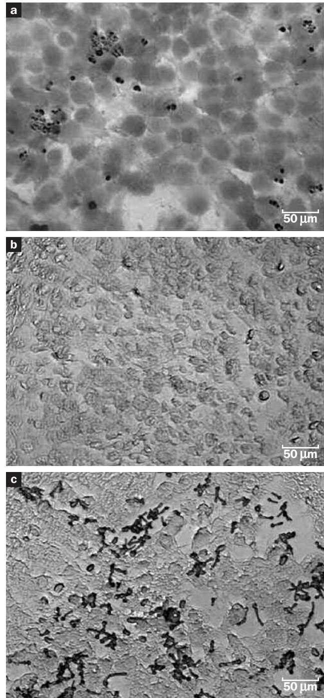
Fig. 1. Phase contrast images of the steps of the proposed method: a) yeasts and TCC-SUP cells stained with CV only; b) TCC-SUP cells destained with ethanol and acetone; c) Yeast cells stained strongly with crystal violet and TCC-SUP cells destained with ethanol and acetone (original magnification x200).
