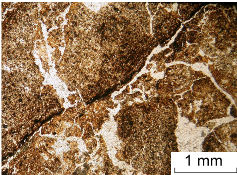
Figure 4c. PPL.
