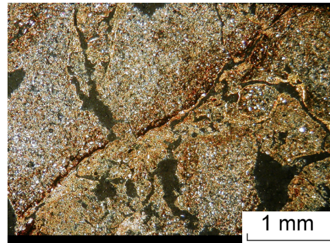
Figure 4d. XPL.
